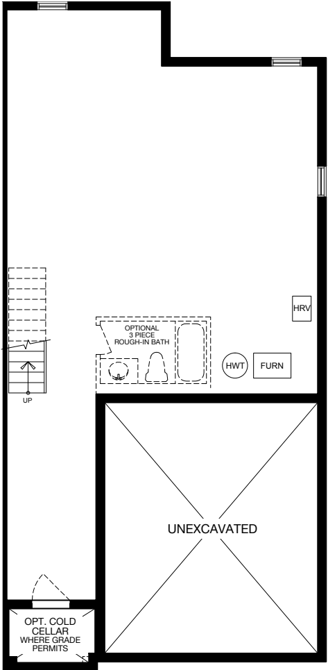
BASEMENT PLAN
