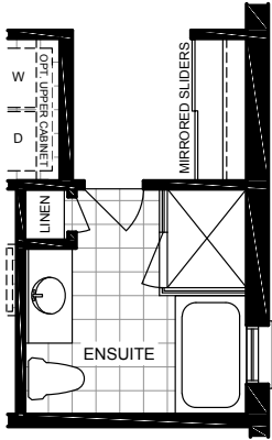
OPTIONAL ENSUITE LAYOUT WITH BATHTUB
