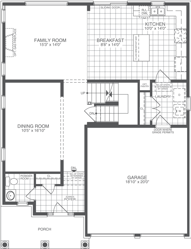
FIRST FLOOR ELEVATION A & B
