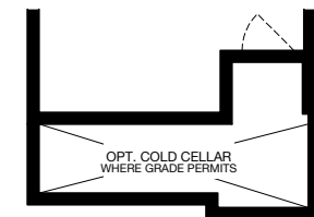
BASEMENT PLAN ELEVATION B
