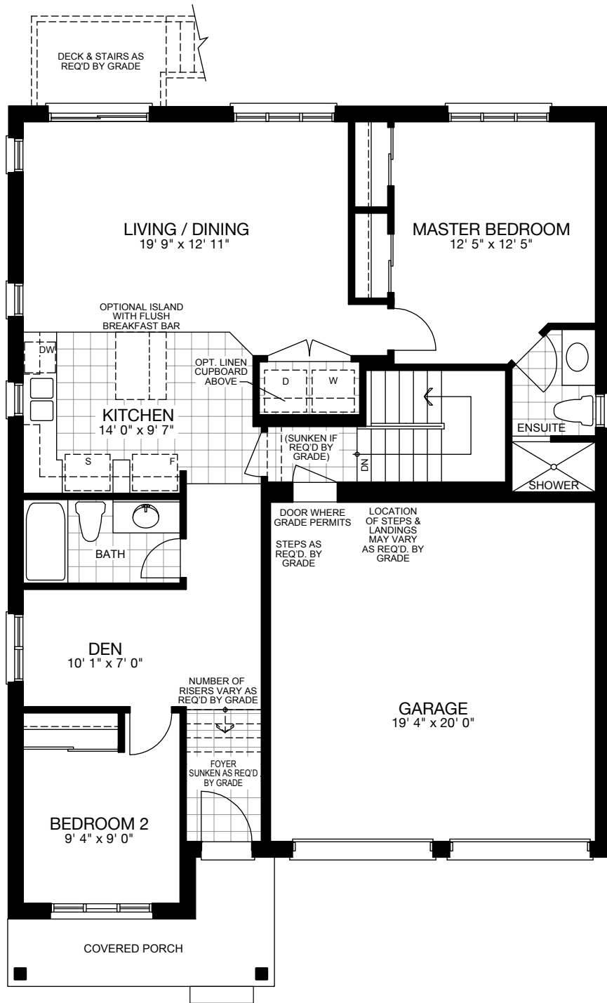
9' CEILING GROUND FLOOR PLAN
