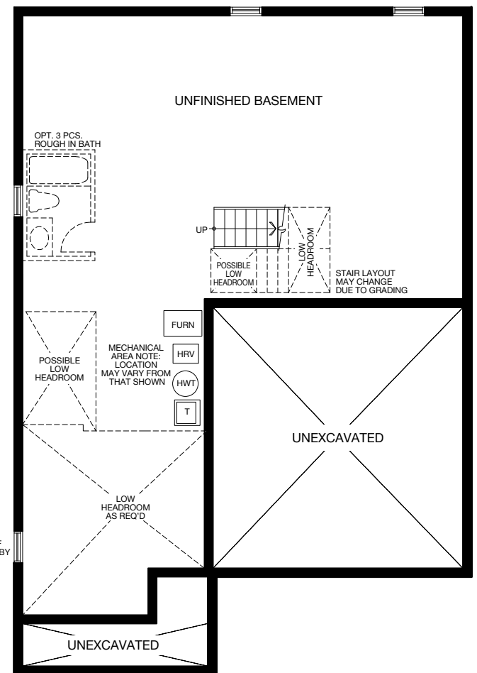
BASEMENT PLAN
