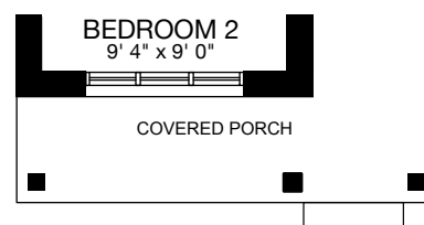
PARTIAL GROUND FLOOR PLAN ELEVATION B
